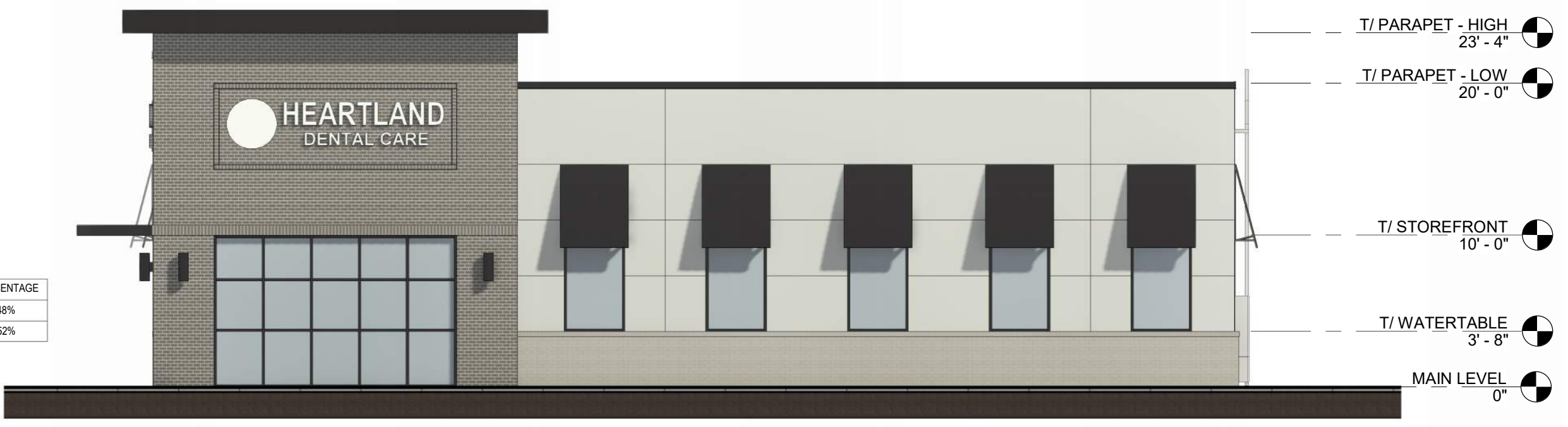
WEST ELEVATION
