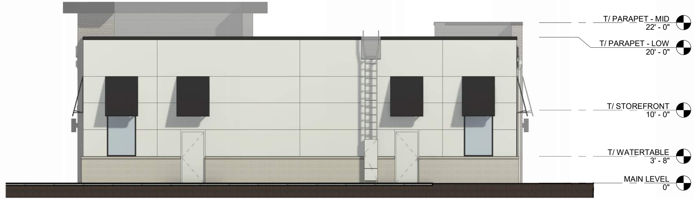
NORTH ELEVATION
